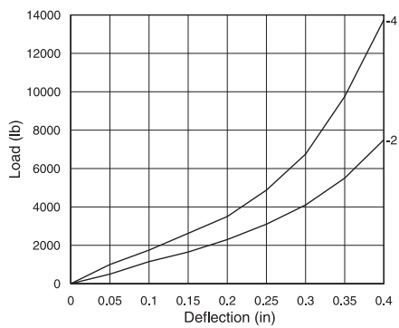
BC1125 Series Axial Load vs. Deflection
