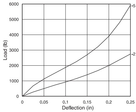
BC1124 Series Axial Load vs. Deflection
