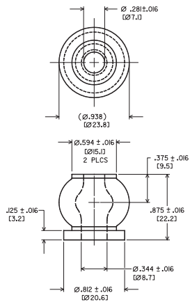
372 Series Dimensional Drawing
